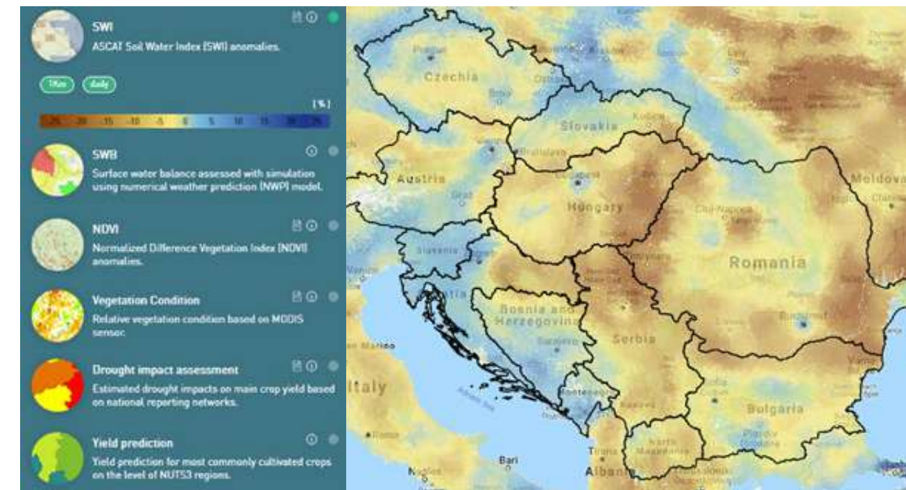
Soil Water Index as seen in Drought Watch on 9 April 2019
